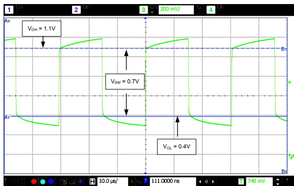
NanoDrive TM Output Waveform (V OH = 1.1V, V OL = 0.4V; SiT1532AI-J4-D14-32.768)
