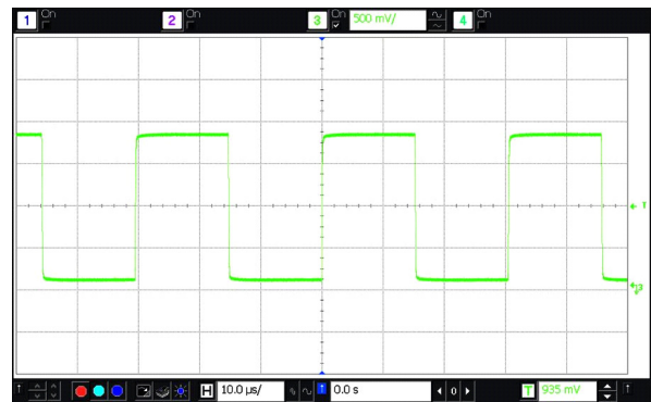
LVC MOS Output Waveform (V swing = 1.8V, SiT1532AI-J4-DCC-32.768)
